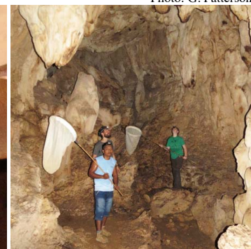
15 Limestone Caves
